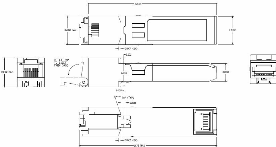
Figure 2. TISTMRR-CNS1 mechanical dimensions
